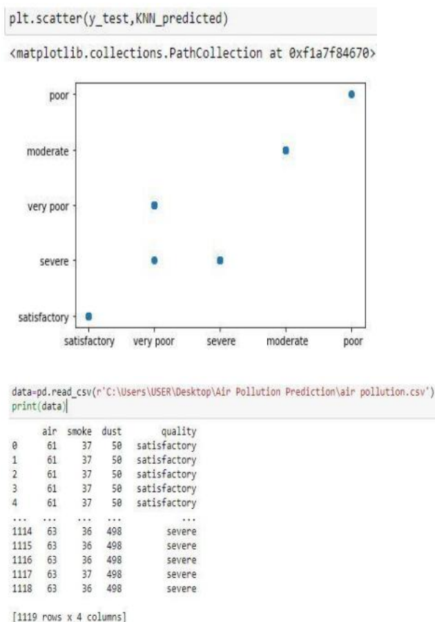
Fig.1. Dataset details.
